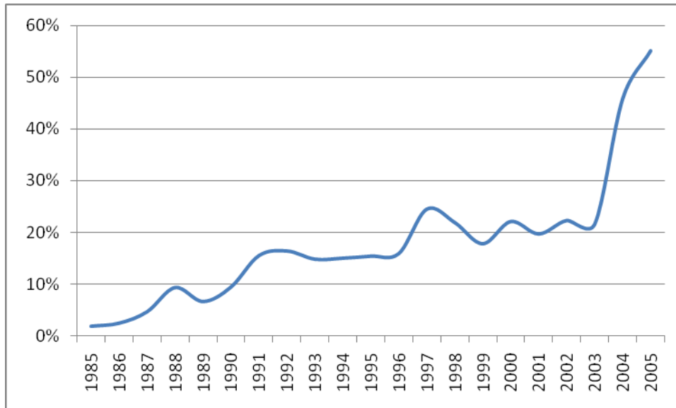
Figure 8a: Market Share of Non-Agency (not Fannie Mae, Freddie Mac or Ginnie Mae) Securitization
