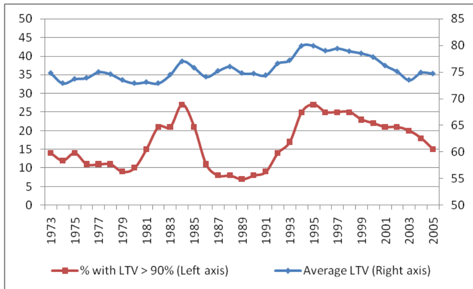
Figure 6: Loan-to-Value Ratio Trends (%)
