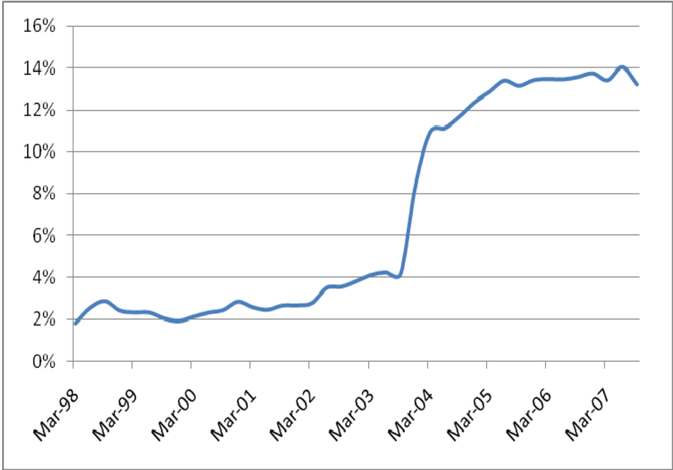
Figure 8: Subprime Share as a Percent of Total Serviced Loans
