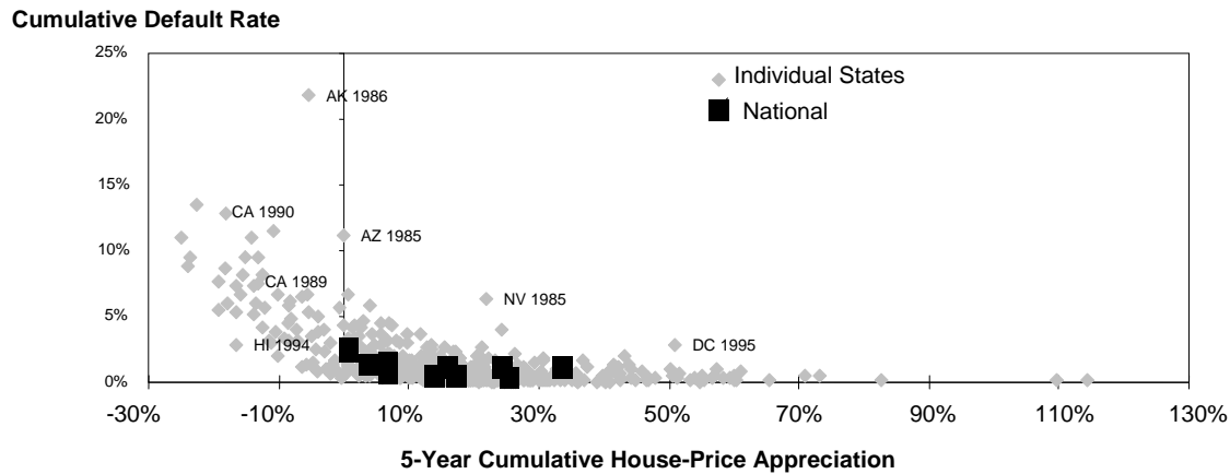
Figure 3: Default Probability versus House Price Appreciation by Origination Year: The figure plots the cumulative default rates for 80% Loan-to-Value, 30-Year Fixed-Rate Home-Purchase Mortgages from 1985-1995 for both states and national data.
